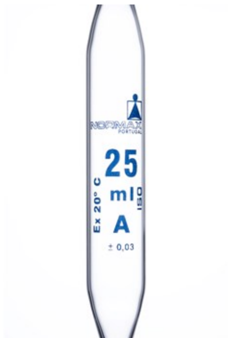
Volumetric pipette 2 marks, blue printing, class AS, Normax 25 ml
